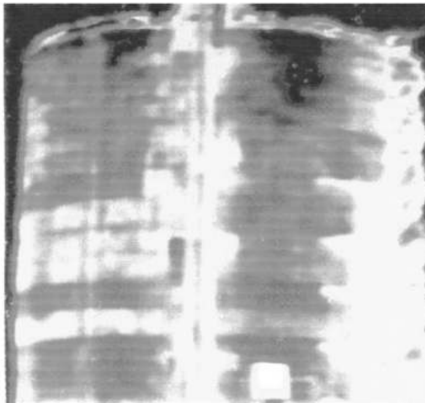
Figure 2. Thermogram of the ethylene vessel.
