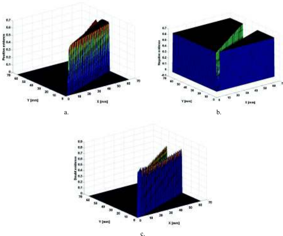
Figure 5. The evidence for ultrasound beam with centre in C_1 : a) positive evidence; b) negative evidence; c) doubt evidence
