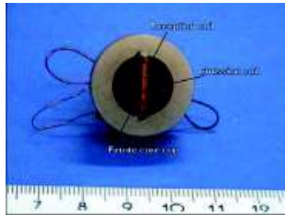
Figure 7. Eddy current transducer with orthogonal coils
