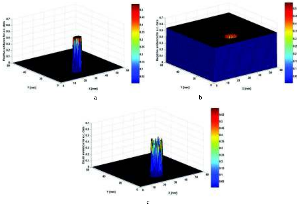
Figure 10. The evidence for eddy current examination: a) positive evidence; b) negative evidence; c) doubt evidence
