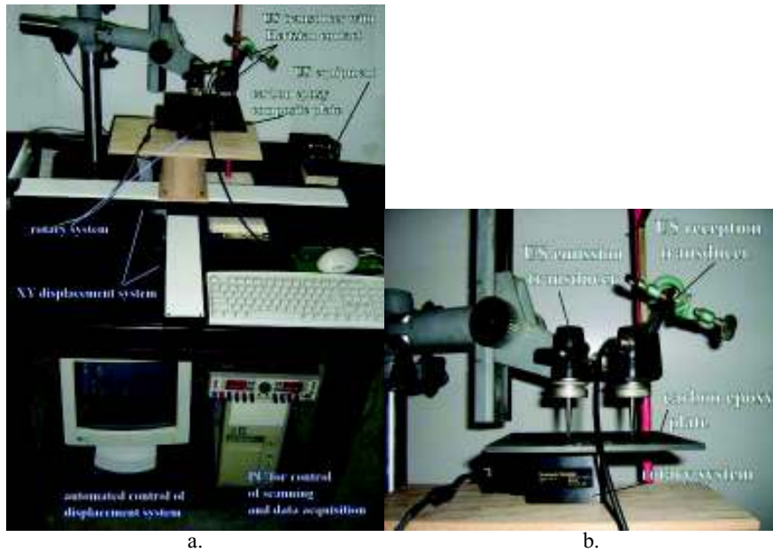
Figure 2 Experimental set-up: a) Equipment; b) US transducers
