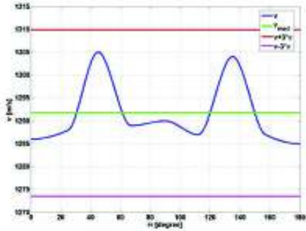
Figure 3. The angular dependency of US propagation speed on a zone without delamination
