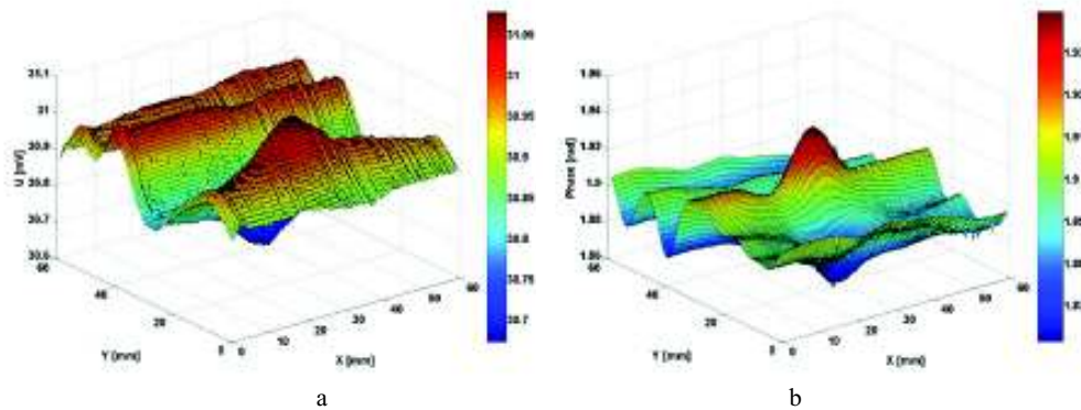
Figure 8. Eddy current signal at the scanning over a delamination: a) amplitude; b) phase
