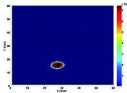
Figure 9. Eddy current holography
