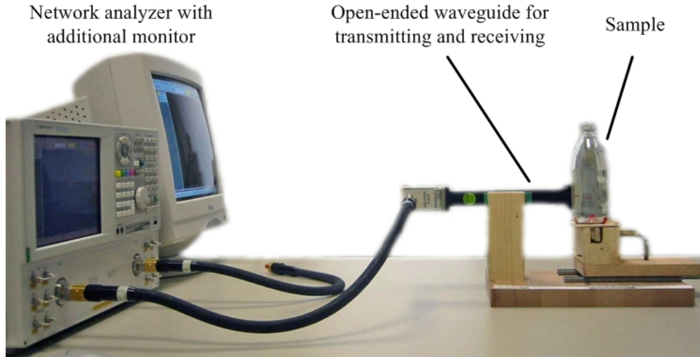
Fig. 1: Measurement Setup
