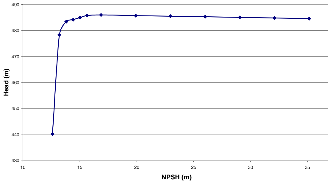
Figure 4 Deferential Head vs. NPSH at flow rate 1686 meter 3 / h
