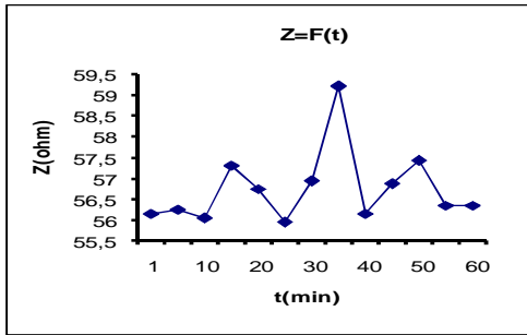
Figure 1: impedance according to solicitation time (charge F1),Al
