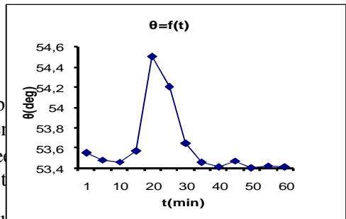
Figure 8: Phase according to solicitation time (case continue, charge F2),Al
