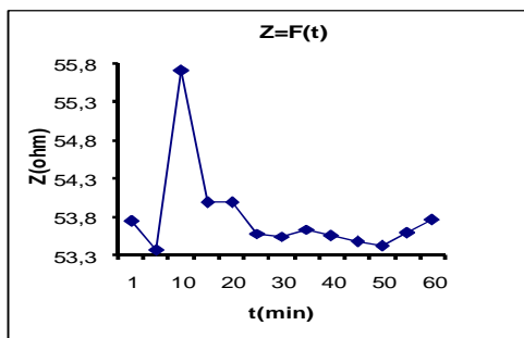
Figure 9: Impedance according to solicitation time (charge F1, stainless steel)
