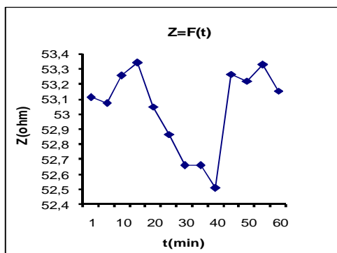
Figure 11: Impedance according to solicitation time (charge F1, E24)
