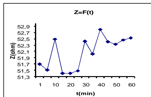
Figure 10: Impedance according to solicitation time (charge F2, stainless steel)
