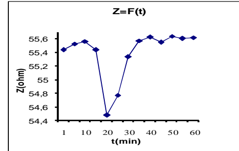
Figure 6: Impedance according to solicitation time (charge continue, 2),Al
