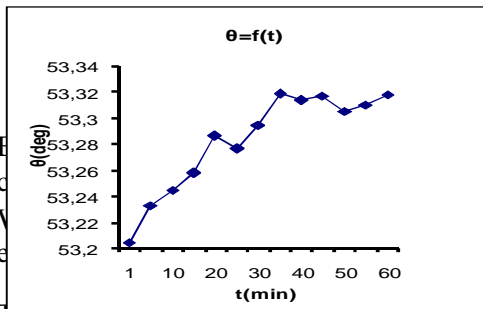
Figure 7: Phase according to solicitation time (case continue, charge F1) Al
