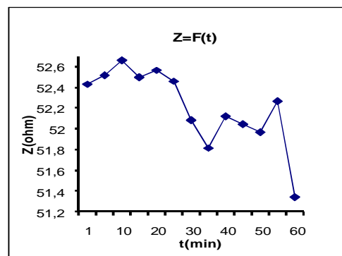
Figure 11: Impedance according to solicitation time (charge F2, E24)
