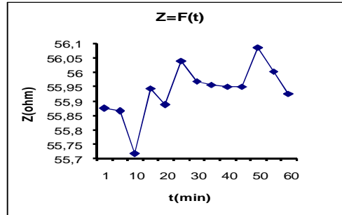
Figure 2: impedance according to solicitation time (charge F2),Al
