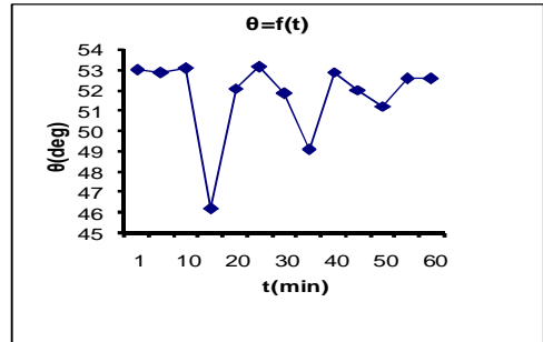
Figure 4: Phase according to solicitation time (charge F2),Al
