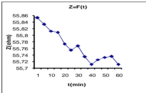
Figure 5: Impedance according to solicitation time (charge continue, F1),Al
