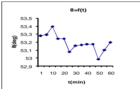
Figure 3: Phase according to solicitation time (charge F1),Al
