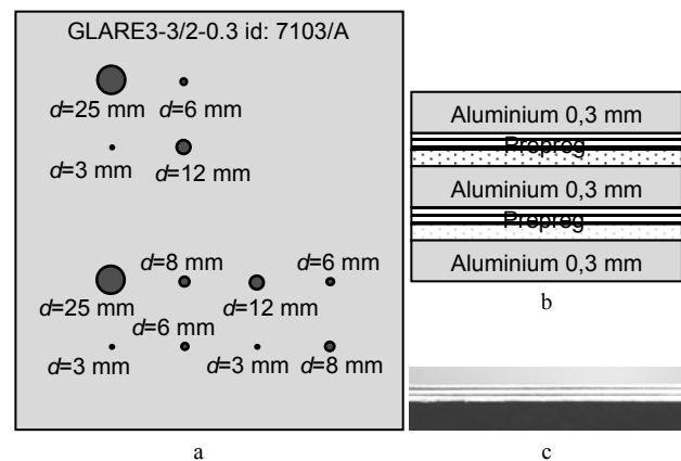
Fig. 1. GLARE3-3/2 test sample (a); drawing of the cross – section of the test sample (b); image of the cross – section of the test sample (c);
