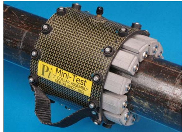
Figure - 3" Mini-Tool assembly
